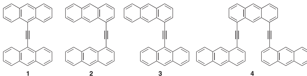
Figure 1. Structures of target anthrylethynes.
