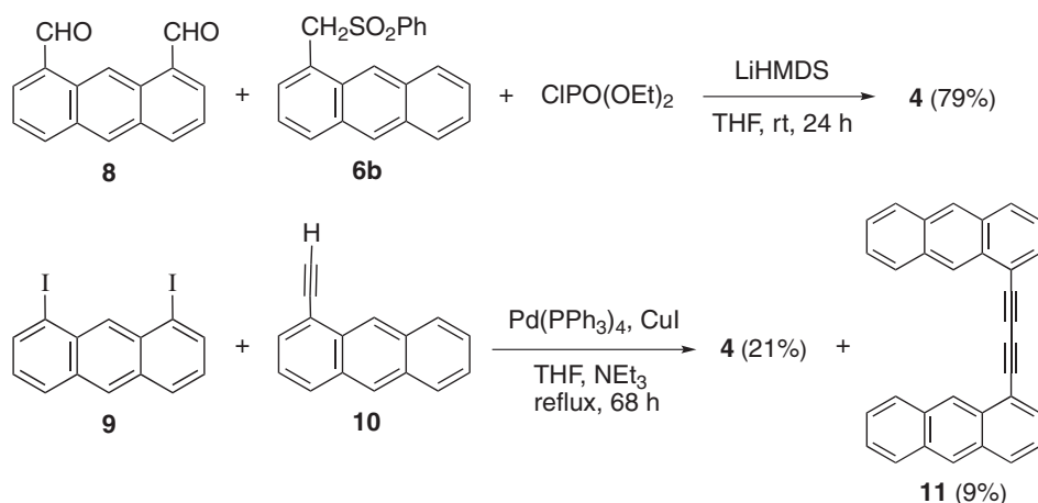
Scheme 3. Synthesis of anthrylene-ethynylene trimer 4 by one-shot double elimination and Sonogashira coupling.
