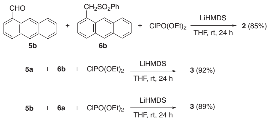
Scheme 2. Synthesis of dianthrylethyne 2 and 3 by one-shot double elimination.
