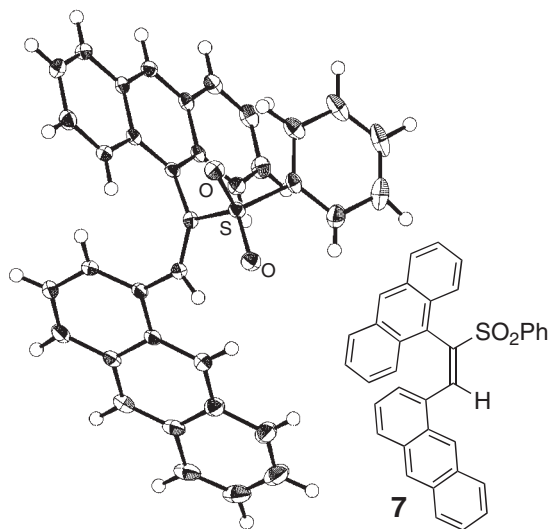
Figure 2. ORTEP drawing of vinyl sulfone 7 . Solvent molecules are omitted for clarity.
